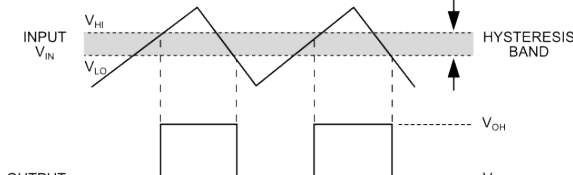
Figure 8: Analog Comparator Hysteresis Band and Output Switching Points.
